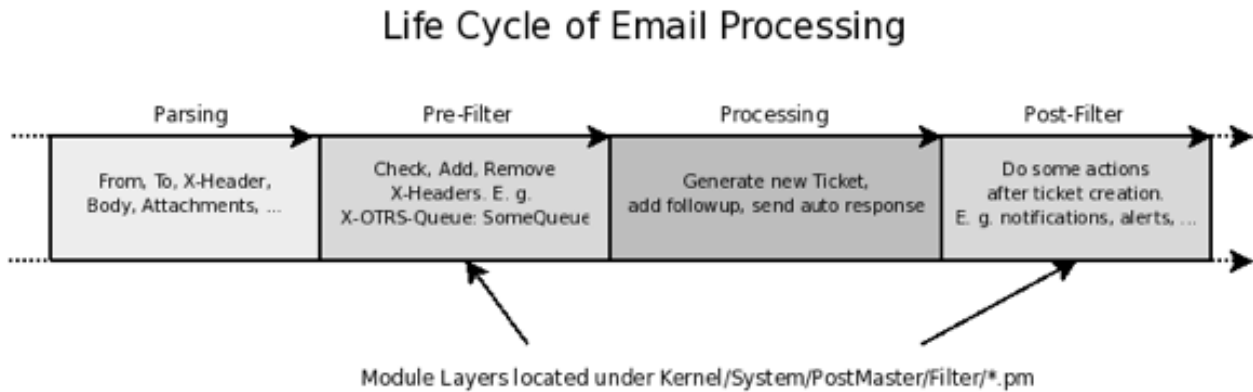
Fig. 3.6: Email Processing Flow
