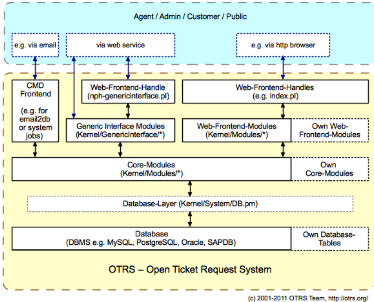
Fig. 1.1: OTOBO Architecture
